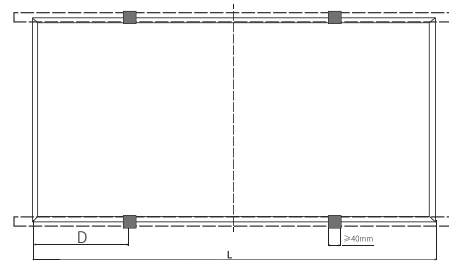
clamp installation (clamp length \geq 40\text{mm} )
