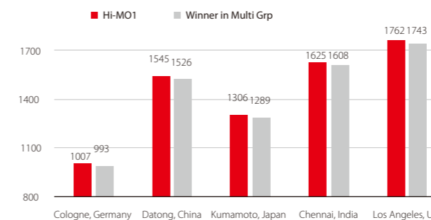
Simulated Power Generation (kWh/kWp/year)
