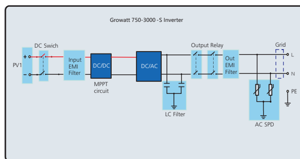
Growatt 750-3000 -S topology
